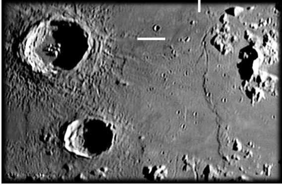
Fig. 3: Dome Ari1 near the crater Aristillus. Telescopic CCD image acquired on October 26, 2009, at 18:05 UT.
