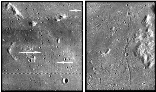
Fig. 4: Left: Lunar Orbiter image IV-168-H3. Arrows indicate short rilles on the surface of Gr1. Right: Lunar Orbiter image IV-110-H1, showing straight rilles on the surface of Ari1.
